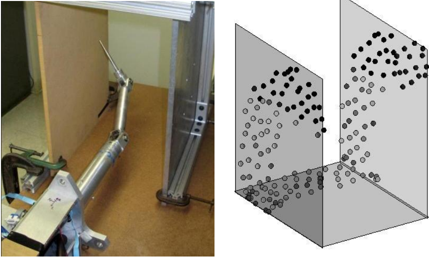
Fig. 9. (Left) Three-planes environment for the evaluation of joint backlash. (Right) Touched points and reconstructed surface. The intensity of the points represents the magnitude of the backlash correction for the first link.
