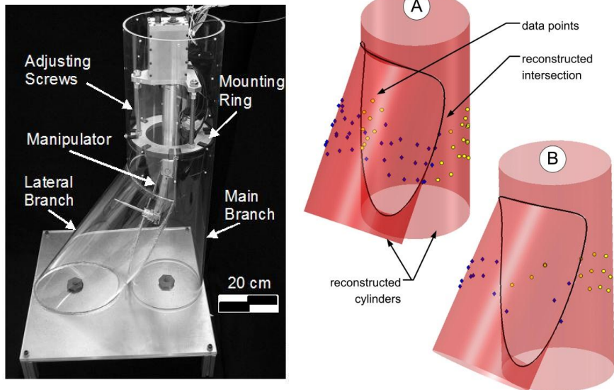
Fig. 6. (Left) Plexiglas tank reproducing an oil well junction, with tactile manipulator. (Right) Result of the exploration using (A) a uniform sampling and (B) the algorithm developed in this work: the number of required points decreases.
