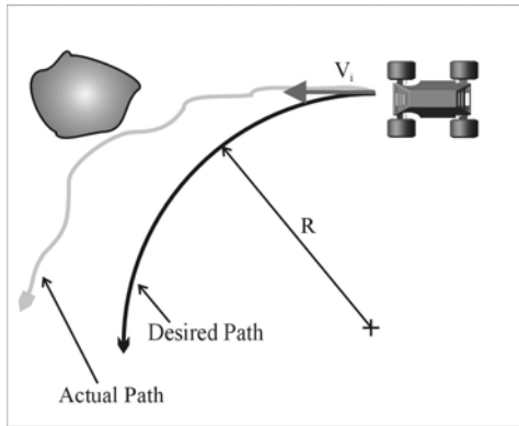
Figure 3. Schematic of the high-speed turn analysis.
