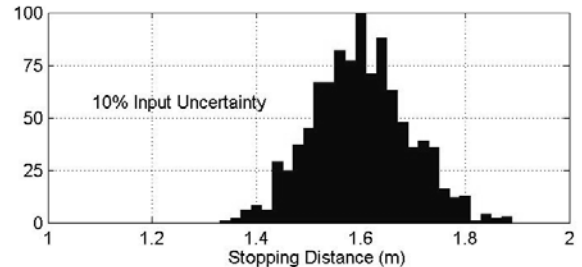
Figure 4. Stopping distance distribution for 10% uniform parameter uncertainty
