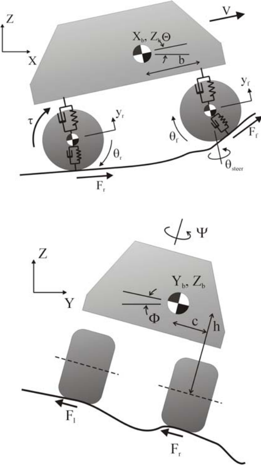
Figure 1. Schematic of high-speed mobile robot model.
