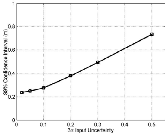
Figure 5. Stopping distance vs. parameter input uncertainty
