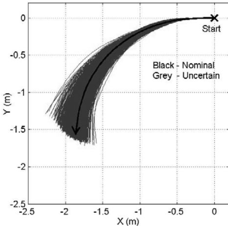
Figure 6. Uncertain turn trajectories; n = 1000 , u = 0.2 .
