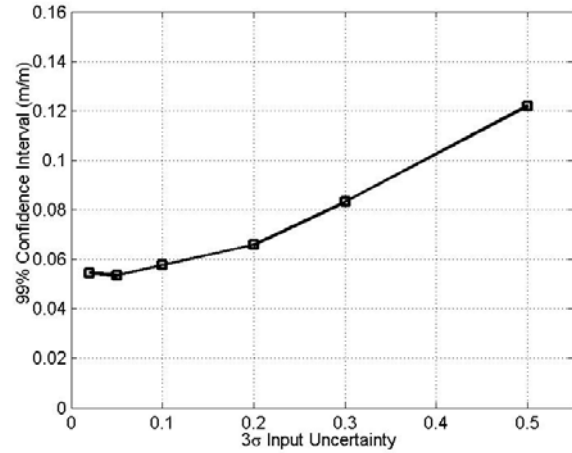
Figure 7. High-speed turning error uncertainty.
