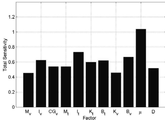
Figure 9. High-speed turning total sensitivity indices.
