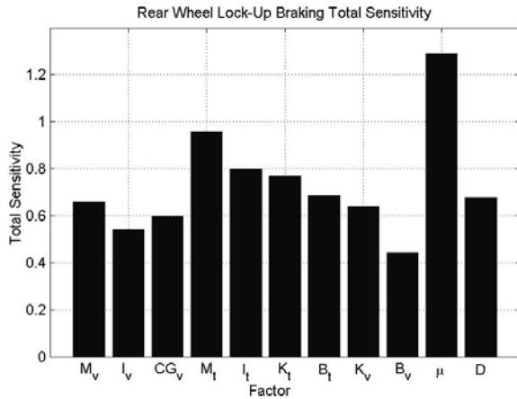
Figure 8. Braking maneuver total sensitivity indices.
